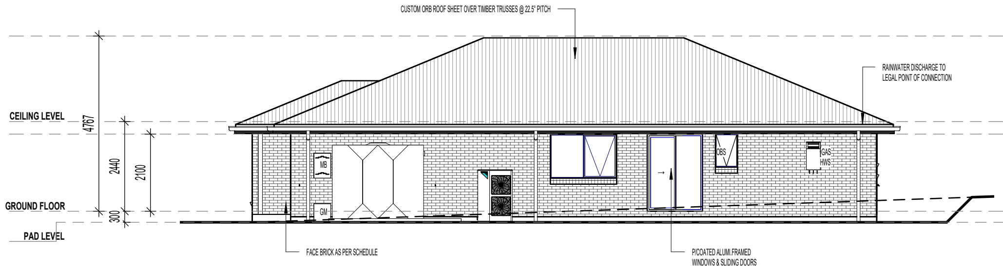
EASTERN ELEVATION 1 : 100
