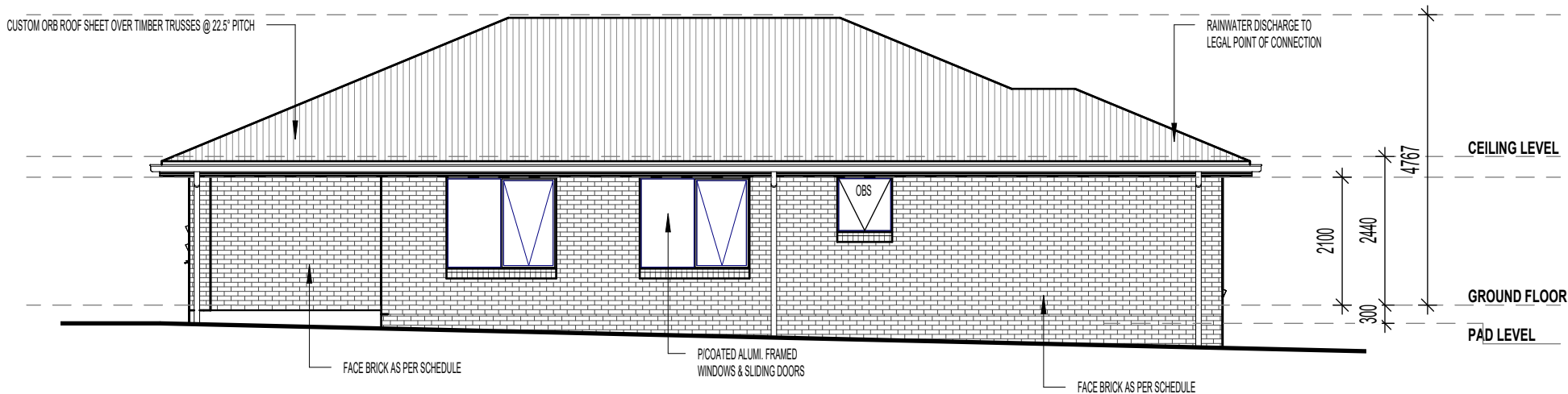
WESTERN ELEVATION 1 : 100
