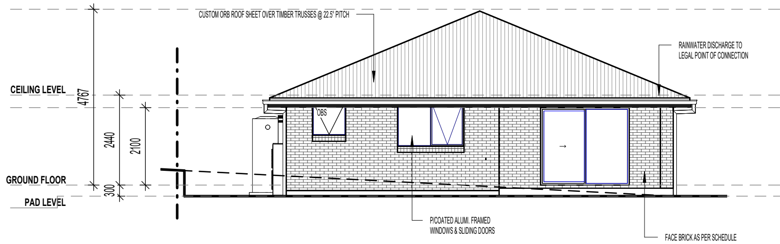
NORTHERN ELEVATION 1 : 100
