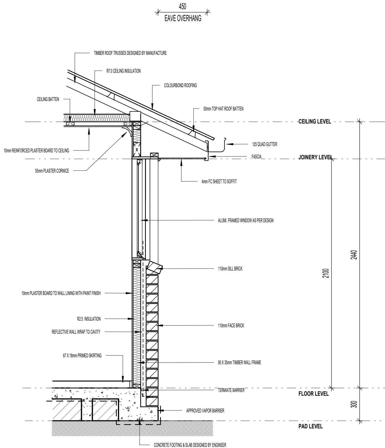
TYP. BRICK VENEER WALL DETAIL - CB ROOF 1 : 20
